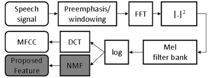
図 1 Feature extraction flow
