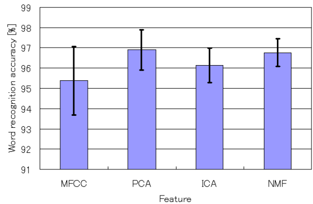
図 7 Comparison of MFCC, PCA, ICA and NMF speech features.
