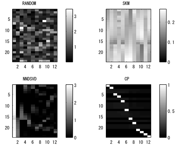
図 2 W by NMF initialization: RANDOM, SKM, NNDSVD, and CP.
