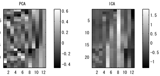
図 6 W by PCA (left) or ICA(right).
