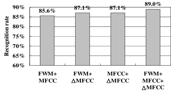
Figure 8. Results of speaker independent phoneme recognition by feature integration.
