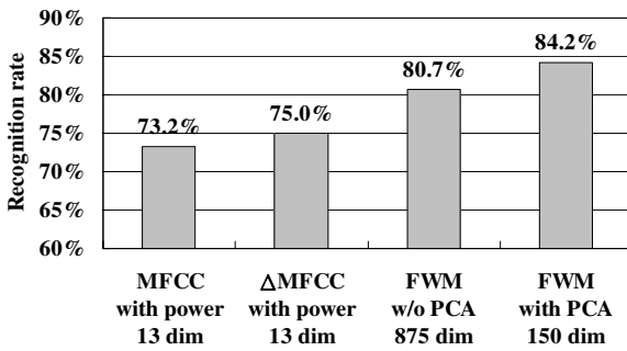
Figure 7. Results of speaker independent phoneme recognition by single feature.
