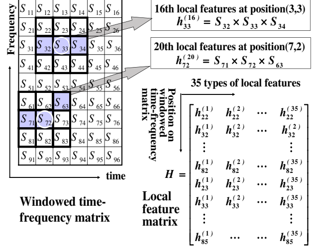
Figure 4. Local feature matrix.
