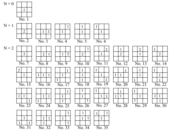
Figure 3. 35 types of local patterns.
