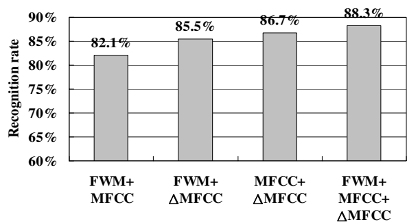
Figure 6. Results of speaker dependent phoneme recognition by feature integration.
