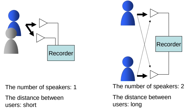
図6 パワーを元にした特徴量で判別できない例 Fig. 6 An example in which the power based system cannot detect speakers correctly.
