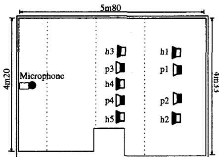
Figure 2. A top view of the experimental room
