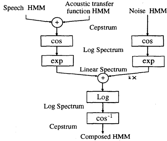
Figure 1. Block Diagram of HMM Composition
